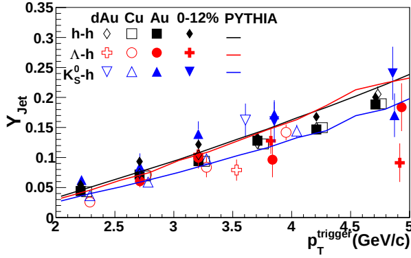
FIG. 2: The jet-like yield in |\Delta\eta| < 0.78 as a function of p_T^{\text{trigger}} for h-h [14], K_S^0 -h, and \Lambda -h correlations for 1.5 \text{ GeV}/c < p_T^{\text{associated}} < p_T^{\text{trigger}} in d+Au, Cu+Cu, and Au+Au collisions at \sqrt{s_{NN}} = 200 \text{ GeV} . The data from Au+Au collisions are shown in two centrality bins, 40-80% and 0-12%. The data are compared to PYTHIA [32] calculations using the Perugia 2011 tune [33].
