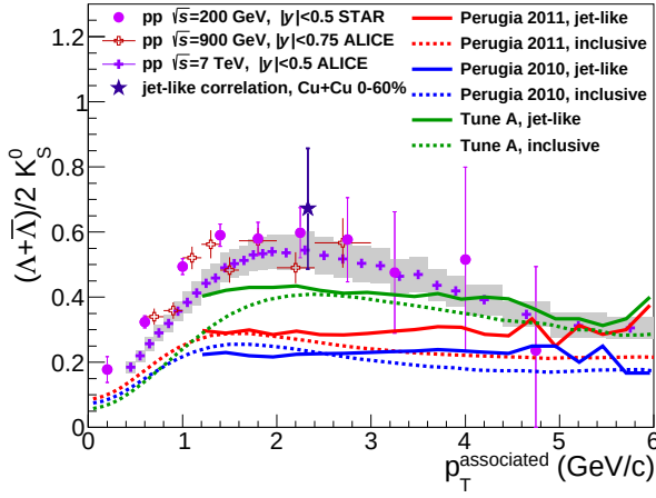
FIG. 5: \Lambda/K_S^0 ratio measured in the jet-like correlation in Cu+Cu collisions at \sqrt{s_{NN}} = 200 GeV for 3 < p_T^{\text{trigger}} < 6 GeV/c and 2.0 < p_T^{\text{associated}} < 3.0 GeV/c along with this ratio obtained from inclusive p_T spectra in p+p collisions.
