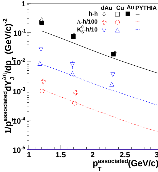
FIG. 4: The jet-like yield as a function of p_T^{\text{associated}} for h-h [14], K_S^0 -h, and \Lambda -h correlations for 3 < p_T^{\text{trigger}} < 6 GeV/c in d+Au, Cu+Cu, and Au+Au collisions at \sqrt{s_{NN}} = 200 GeV. The data are compared to PYTHIA [32] calculations using the Perugia 2011 tune [33].
