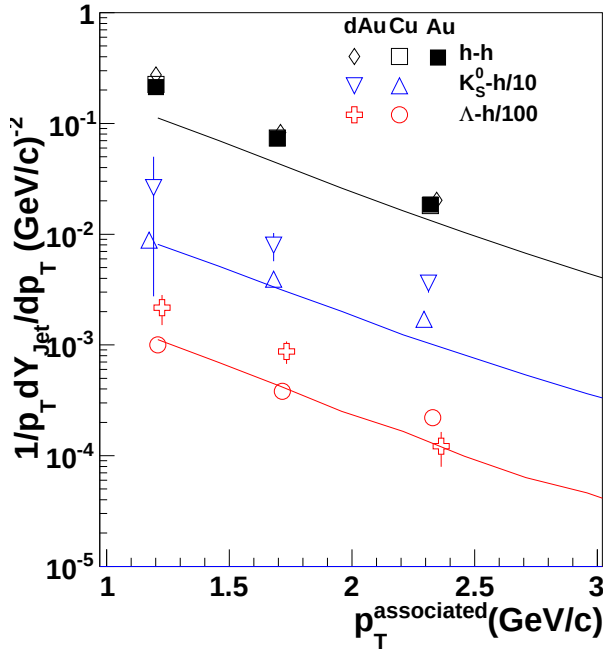
FIG. 3: The jet-like yield as a function of p_T^{\text{associated}} for h-h [19], K_S^0 -h, and \Lambda , \bar{\Lambda} -h correlations in d +Au, Cu+Cu, and Au+Au collisions at \sqrt{s_{NN}} = 200 GeV. The data are compared to PYTHIA [25] calculations using the Perugia 2011 [26] tune [26].
