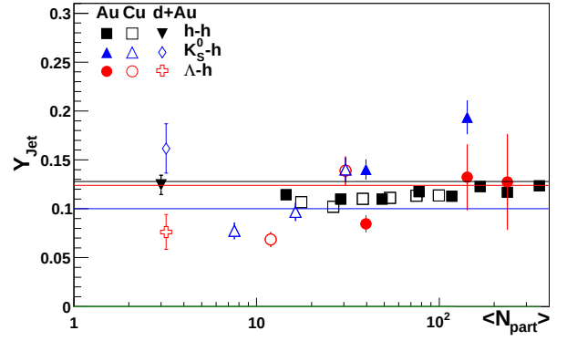
FIG. 2: N_{\text{part}} dependence of the jet-like yield of h-h, K_S^0 -h, and \Lambda , \bar{\Lambda} -h correlations in d+Au, Cu+Cu, and Au+Au collisions at \sqrt{s_{NN}} = 200 GeV. The data from Au+Au collisions are shown in two centrality bins, 40-80% and 0-12%. The data are compared to PYTHIA [25] calculations using the Perugia 2011 tune [26].
