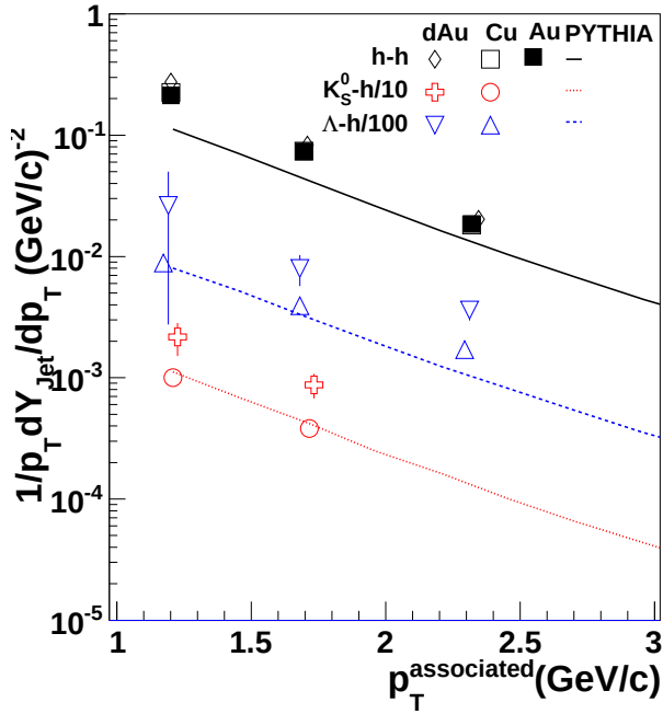
FIG. 4: The jet-like yield as a function of p_T^{\text{associated}} for h-h [14], K_S^0 -h, and \Lambda , \bar{\Lambda} -h correlations in d +Au, Cu+Cu, and Au+Au collisions at \sqrt{s_{NN}} = 200 GeV. The data are compared to PYTHIA [29] calculations using the Perugia 2011 tune [30].
