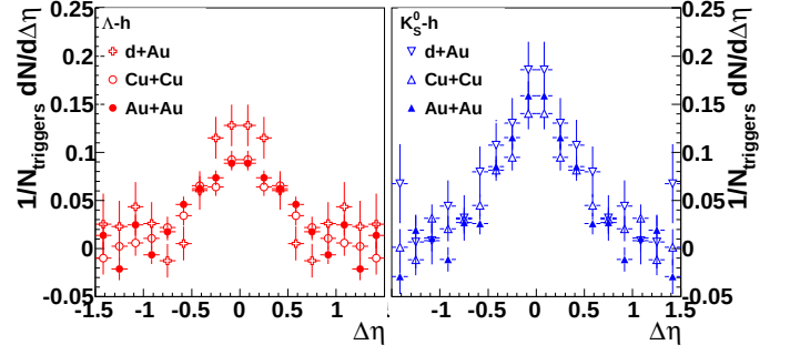
FIG. 1: \frac{dN_J}{d\Delta\eta} for \Lambda, \bar{\Lambda} -h (left) and K_S^0 -h (right) correlations for minimum bias d+Au collisions, 0-20% Cu+Cu collisions, and 40-80% Au+Au correlations. The data have been reflected about \Delta\eta = 0 .
