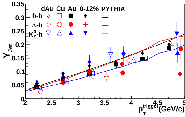
FIG. 2: The jet-like yield in |\Delta\eta| < 0.78 as a function of p_T^{\text{trigger}} for h-h [14], K_S^0 -h, and \Lambda, \bar{\Lambda} -h correlations for 1.5 \text{ GeV}/c < p_T^{\text{associated}} < p_T^{\text{trigger}} in d+Au, Cu+Cu, and Au+Au collisions at \sqrt{s_{NN}} = 200 \text{ GeV} . The data from Au+Au collisions are shown in two centrality bins, 40-80% and 0-12%. The data are compared to PYTHIA [31] calculations using the Perugia 2011 tune [32].
