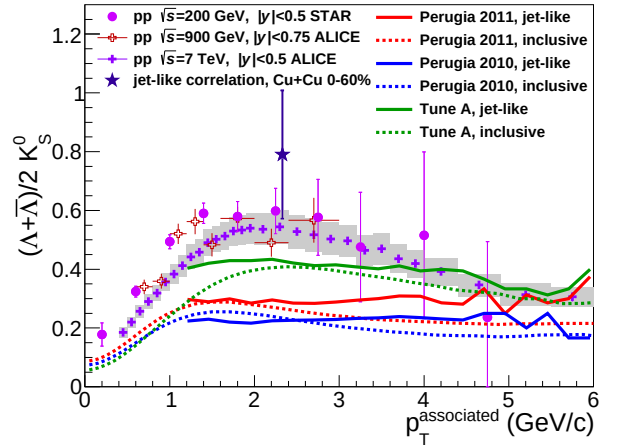
FIG. 5: \Lambda/K_S^0 ratio measured in the jet-like correlation in Cu+Cu collisions at \sqrt{s_{NN}} = 200 GeV for 3 < p_T^{\text{trigger}} < 6 GeV/c and 2.0 < p_T^{\text{associated}} < 3.0 GeV/c along with this ratio obtained from inclusive p_T spectra in p+p collisions.
