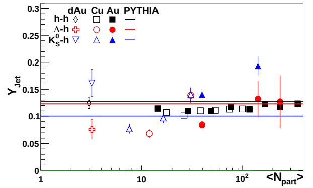
FIG. 3: Centrality dependence of the jet-like yield of h-h, K_S^0 -h, and \Lambda, \bar{\Lambda} -h correlations for 3 < p_T^{\text{trigger}} < 6 \text{ GeV}/c and 1.5 \text{ GeV}/c < p_T^{\text{associated}} < p_T^{\text{trigger}} in d+Au, Cu+Cu, and Au+Au collisions at \sqrt{s_{NN}} = 200 \text{ GeV} . The data from Au+Au collisions are shown in two centrality bins, 40-80% and 0-12%. The data are compared to PYTHIA [31] calculations using the Perugia 2011 tune [32].
