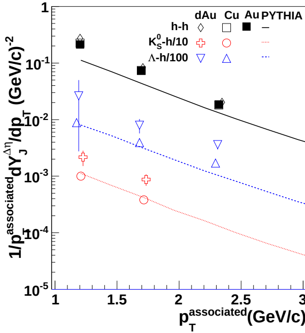
FIG. 4: The jet-like yield as a function of p_T^{\text{associated}} for h-h [14], K_S^0 -h, and \Lambda, \bar{\Lambda} -h correlations for 3 < p_T^{\text{trigger}} < 6 GeV/c in d+Au, Cu+Cu, and Au+Au collisions at \sqrt{s_{NN}} = 200 GeV. The data are compared to PYTHIA [31] calculations using the Perugia 2011 tune [32].
