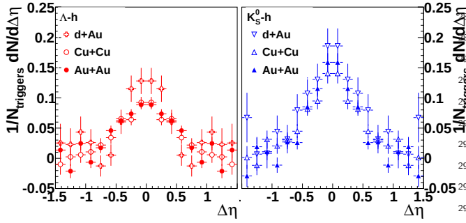
FIG. 1: Corrected correlation functions \frac{dN_J}{d\Delta\eta} in |\Delta\phi| = 1.0 for 3 < p_T^{\text{trigger}} < 6 GeV/c and 1.5 GeV/c < p_T^{\text{associated}} < p_T^{\text{trigger}} for \Lambda -h (left) and K_S^0 -h (right) for minimum bias d +Au, 0-20% Cu+Cu, and 40-80% Au+Au collisions at \sqrt{s_{NN}} = 200 GeV after background subtraction. The data have been reflected about \Delta\eta = 0 .
