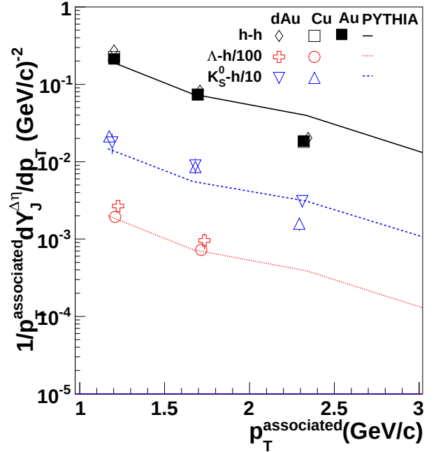
FIG. 5: The jet-like yield as a function of p_T^{\text{associated}} for h-h [7], K_S^0 -h, and \Lambda -h correlations for 3 < p_T^{\text{trigger}} < 6 \text{ GeV}/c in d+Au, 0-60% Cu+Cu, and 40-80% Au+Au collisions at \sqrt{s_{NN}} = 200 \text{ GeV} . The data are compared to PYTHIA [35] calculations using the Perugia 2011 tune [36]. Data are binned in 1.0 < p_T^{\text{associated}} < 1.5 \text{ GeV}/c , 1.5 < p_T^{\text{associated}} < 2.0 \text{ GeV}/c , and 2.0 < p_T^{\text{associated}} < 3.0 \text{ GeV}/c and are plotted at the mean of the bin.
