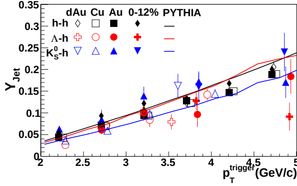
FIG. 3: The jet-like yield in |\Delta\eta| < 0.78 as a function of p_T^{\text{trigger}} for h-h [7], K_S^0 -h, and \Lambda -h correlations for 1.5 \text{ GeV}/c < p_T^{\text{associated}} < p_T^{\text{trigger}} in minimum bias d+Au, 0-60% Cu+Cu, and Au+Au collisions at \sqrt{s_{NN}} = 200 \text{ GeV} . The data from Au+Au collisions are shown in two centrality bins, 40-80% and 0-12%. The data are compared to PYTHIA [35] calculations using the Perugia 2011 tune [36]. Data have been offset for visibility.
