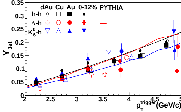
FIG. 3: The jet-like yield in |\Delta\eta| < 0.78 as a function of p_T^{\text{trigger}} for h-h [7], K_S^0 -h, and \Lambda -h correlations for 1.5 GeV/c < p_T^{\text{associated}} < p_T^{\text{trigger}} in minimum bias d+Au, 0-60% Cu+Cu, and Au+Au collisions at \sqrt{s_{NN}} = 200 GeV. The data from Au+Au collisions are shown in two centrality bins, 40-80% and 0-12%. The data are compared to PYTHIA [36] calculations using the Perugia 2011 tune [37]. Data have been offset for visibility. The 5% systematic error due to the uncertainty on the associated particle's efficiency is not shown.
