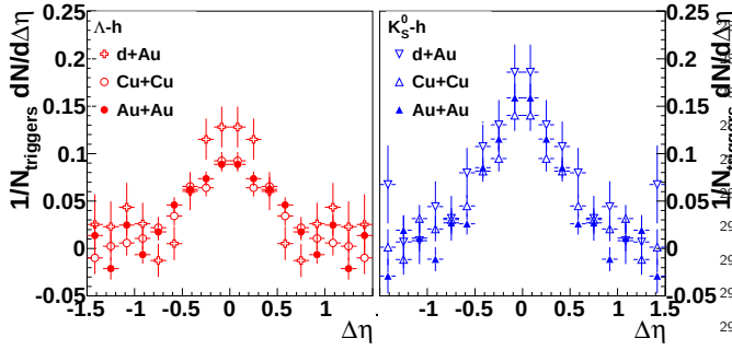
FIG. 1: Corrected correlation functions \frac{dN}{d\Delta\eta} in |\Delta\phi| = 1.0 for 3 < p_T^{\text{trigger}} < 6 GeV/c and 1.5 GeV/c < p_T^{\text{associated}} < p_T^{\text{trigger}} for \Lambda -h (left) and K_S^0 -h (right) for minimum bias d +Au, 0-20% Cu+Cu, and 40-80% Au+Au collisions at \sqrt{s_{NN}} = 200 GeV after background subtraction. The data have been reflected about \Delta\eta = 0 .
