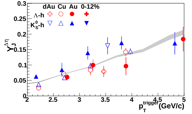
FIG. 4: The jet-like yield in |\Delta\eta| < 0.78 as a function of p_T^{\text{trigger}} for K_S^0 -h, and \Lambda -h correlations for 1.5 \text{ GeV}/c < p_T^{\text{associated}} < p_T^{\text{trigger}} in minimum bias d+Au, 0-60% Cu+Cu, and Au+Au collisions at \sqrt{s_{NN}} = 200 GeV. The data from Au+Au collisions are shown in two centrality bins, 40-80% and 0-12%. For comparison h-h correlations [7] from 40-80% Au+Au collisions are shown as a band where the width represents the error. Peripheral Au+Au points have been shifted in p_T^{\text{trigger}} for visibility. The 5% systematic error due to the uncertainty on the associated particle's efficiency is not shown.
