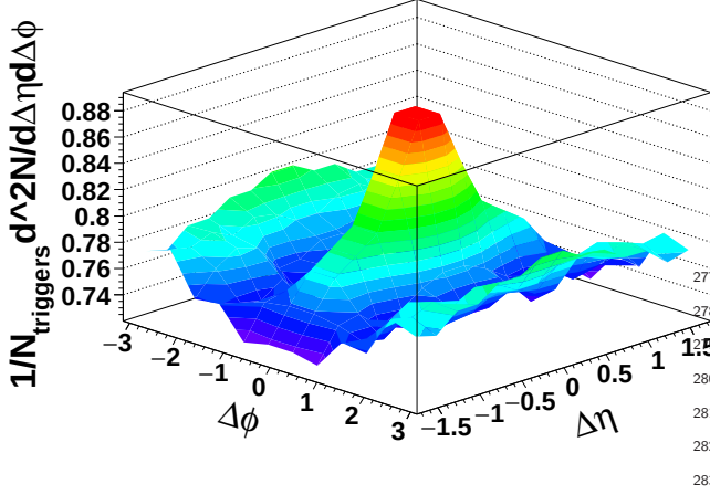
FIG. 1: Corrected 2D K_S^0 -h correlation function for 3 < p_T^{\text{trigger}} < 6 GeV/c and 1.5 GeV/c < p_T^{\text{associated}} < p_T^{\text{trigger}} for 0-20% Cu+Cu. The data have been reflected about \Delta\eta = 0 and \Delta\phi = 0 .
