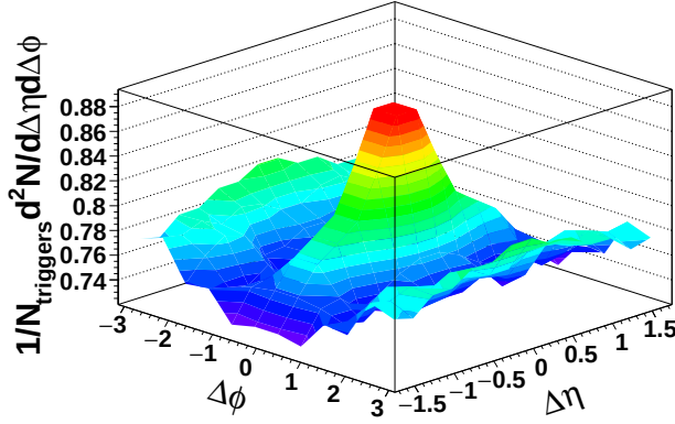
FIG. 1: Corrected 2D K_S^0 -h correlation function for 3 < p_T^{\text{trigger}} < 6 GeV/c and 1.5 GeV/c < p_T^{\text{associated}} < p_T^{\text{trigger}} for 0-20% Cu+Cu. The data have been reflected about \Delta\eta = 0 and \Delta\phi = 0 .
