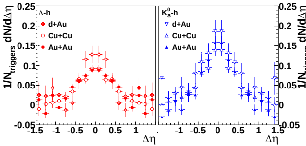
FIG. 2: Corrected correlation functions \frac{dN_J}{d\Delta\eta} in |\Delta\phi| = 1.0 for 3 < p_T^{\text{trigger}} < 6 GeV/c and 1.5 GeV/c < p_T^{\text{associated}} < p_T^{\text{trigger}} for \Lambda -h (left) and K_S^0 -h (right) for minimum bias d+Au, 0-20% Cu+Cu, and 40-80% Au+Au collisions at \sqrt{s_{NN}} = 200 GeV after background subtraction. The data have been reflected about \Delta\eta = 0 .
