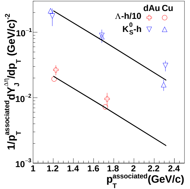
FIG. 6: The jet-like yield as a function of p_T^{\text{associated}} for K_S^0 -h, and \Lambda -h correlations for 3 < p_T^{\text{trigger}} < 6 \text{ GeV}/c in d+Au and 0-60% Cu+Cu collisions at \sqrt{s_{NN}} = 200 \text{ GeV} . The data are compared to the jet-like yield from h-h correlations [7] from 40-80% Au+Au collisions are shown as a band where the width represents the error. Data are binned in 1.0 < p_T^{\text{associated}} < 1.5 \text{ GeV}/c , 1.5 < p_T^{\text{associated}} < 2.0 \text{ GeV}/c , and 2.0 < p_T^{\text{associated}} < 3.0 \text{ GeV}/c and are plotted at the mean of the bin. The systematic errors due to the uncertainty on the associated particle's efficiency (5%) and background level extraction (2%) are not shown.
