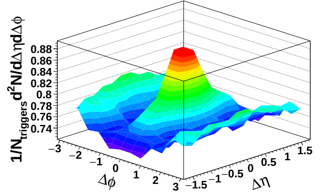
FIG. 1: Corrected 2D K_S^0 -h correlation function for 3 < p_T^{\text{trigger}} < 6 GeV/c and 1.5 GeV/c < p_T^{\text{associated}} < p_T^{\text{trigger}} for 0-20% Cu+Cu. The data have been reflected about \Delta\eta = 0 and \Delta\phi = 0 .
