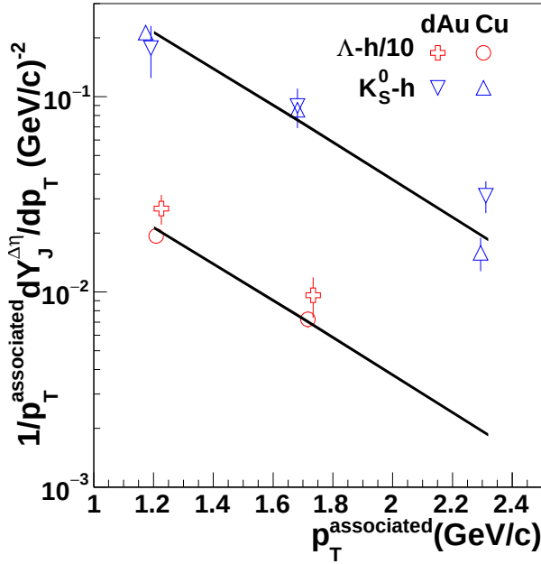
FIG. 6: The jet-like yield as a function of p_T^{\text{associated}} for K_S^0 -h, \Lambda -h, and \Lambda -h correlations for 3 < p_T^{\text{trigger}} < 6 GeV/c in d +Au and 0-60% Cu+Cu collisions at \sqrt{s_{NN}} = 200 GeV. The data are compared to the jet-like yield from h-h correlations [7] from 40-80% Au+Au collisions shown as a band where the width represents the uncertainty. Data are binned in 1.0 < p_T^{\text{associated}} < 1.5 GeV/c, 1.5 < p_T^{\text{associated}} < 2.0 GeV/c, and 2.0 < p_T^{\text{associated}} < 3.0 GeV/c and are plotted at the mean of the bin. The systematic uncertainty due to the uncertainty on the associated particle's reconstruction efficiency (5%) and background level extraction (2%) are not shown.
