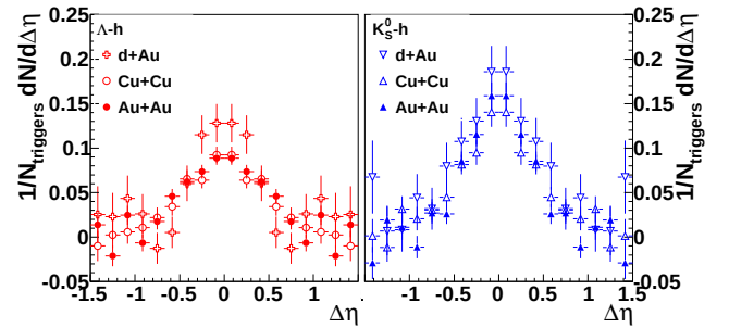
FIG. 2: Corrected correlation functions \frac{dN_I}{d\Delta\eta} in |\Delta\phi| < 0.78 for 3 < p_T^{\text{trigger}} < 6 GeV/c and 1.5 GeV/c < p_T^{\text{associated}} < p_T^{\text{trigger}} for \Lambda -h (left) and K_S^0 -h (right) for minimum bias d+Au, 0-20% Cu+Cu, and 40-80% Au+Au collisions at \sqrt{s_{NN}} = 200 GeV after background subtraction. The data have been reflected about \Delta\eta = 0 .
