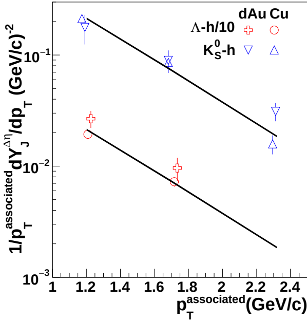
FIG. 6: (Color online.) The jet-like yield as a function of p_T^{\text{associated}} for K_S^0 -h, and \Lambda -h correlations for 3 < p_T^{\text{trigger}} < 6 GeV/c in d+Au and 0-60% Cu+Cu collisions at \sqrt{s_{NN}} = 200 GeV. The data are compared to the jet-like yield from h-h correlations [7] from 40-80% Au+Au collisions shown as a line. Data are binned in 1.0 < p_T^{\text{associated}} < 1.5 GeV/c, 1.5 < p_T^{\text{associated}} < 2.0 GeV/c, and 2.0 < p_T^{\text{associated}} < 3.0 GeV/c and are plotted at the mean of the bin. The systematic uncertainty due to the uncertainty on the associated particle's reconstruction efficiency (5%) and background level extraction (2%) are not shown.
