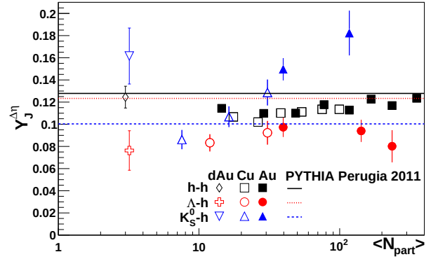
FIG. 5: (Color online.) Centrality dependence of the jet-like yield of K_S^0 -h, and \Lambda -h correlations for 3 < p_T^{\text{trigger}} < 6 GeV/c and 1.5 \text{ GeV/c} < p_T^{\text{associated}} < p_T^{\text{trigger}} in d+Au, Cu+Cu, and Au+Au collisions at \sqrt{s_{NN}} = 200 GeV. The data are compared to PYTHIA [44] calculations using the Perugia 2011 tune [45]. The systematic uncertainty due to the uncertainty on the associated particle's reconstruction efficiency (5%) and background level extraction (2%) are not shown.
