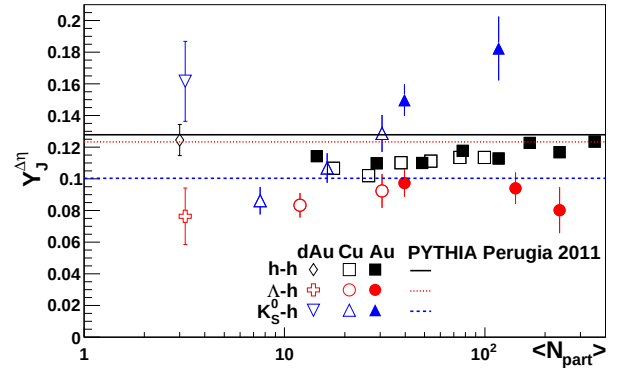
FIG. 5: Centrality dependence of the jet-like yield of K_S^0 -h, and \Lambda -h correlations for 3 < p_T^{\text{trigger}} < 6 GeV/c and 1.5 \text{ GeV}/c < p_T^{\text{associated}} < p_T^{\text{trigger}} in d+Au, Cu+Cu, and Au+Au collisions at \sqrt{s_{NN}} = 200 GeV. The data are compared to PYTHIA [44] calculations using the Perugia 2011 tune [45]. The systematic errors due to the uncertainty on the associated particle's reconstruction efficiency (5%) and background level extraction (2%) are not shown.
