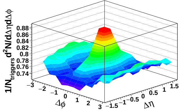
FIG. 1: Corrected 2D K_S^0 -h correlation function for 3 < p_T^{\text{trigger}} < 6 GeV/c and 1.5 \text{ GeV/c} < p_T^{\text{associated}} < p_T^{\text{trigger}} for 0-20% Cu+Cu. The data have been reflected about \Delta\eta = 0 and \Delta\phi = 0 .
