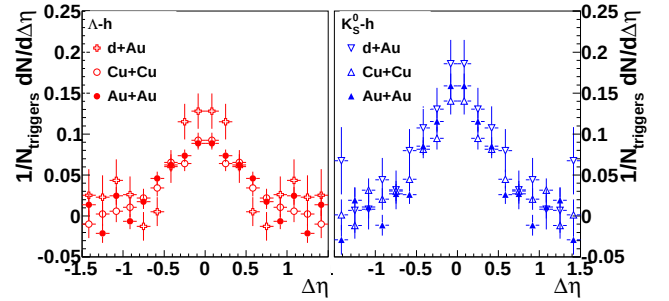
FIG. 2: Corrected correlation functions \frac{dN_I}{d\Delta\eta} in |\Delta\phi| = 1.0 for 3 < p_T^{\text{trigger}} < 6 GeV/c and 1.5 \text{ GeV/c} < p_T^{\text{associated}} < p_T^{\text{trigger}} for \Lambda -h (left) and K_S^0 -h (right) for minimum bias d+Au, 0-20% Cu+Cu, and 40-80% Au+Au collisions at \sqrt{s_{NN}} = 200 GeV after background subtraction. The data have been reflected about \Delta\eta = 0 .
