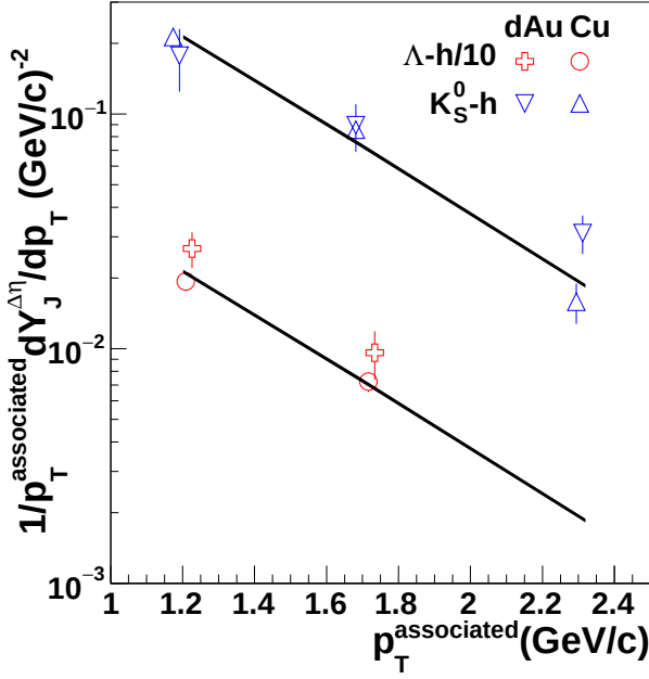
FIG. 5: (Color online.) The jet-like yield as a function of p_T^{\text{associated}} for K_S^0 -h, and \Lambda -h correlations for 3 < p_T^{\text{trigger}} < 6 GeV/c in d+Au and 0-60% Cu+Cu collisions at \sqrt{s_{NN}} = 200 GeV. The data are compared to the jet-like yield from h-h correlations [9] from 40-80% Au+Au collisions shown as a line. Data are binned in 1.0 < p_T^{\text{associated}} < 1.5 GeV/c, 1.5 < p_T^{\text{associated}} < 2.0 GeV/c, and 2.0 < p_T^{\text{associated}} < 3.0 GeV/c and are plotted at the mean of the bin. The systematic uncertainty due to the uncertainty on the associated particle's reconstruction efficiency (5%) and background level extraction (2%) are not shown.
