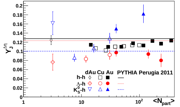
FIG. 4: (Color online.) Centrality dependence of the jet-like yield of K_S^0 -h, and \Lambda -h correlations for 3 < p_T^{\text{trigger}} < 6 GeV/c and 1.5 \text{ GeV/c} < p_T^{\text{associated}} < p_T^{\text{trigger}} in d+Au, Cu+Cu, and Au+Au collisions at \sqrt{s_{NN}} = 200 GeV. The data are compared to PYTHIA [33] calculations using the Perugia 2011 tune [51]. The systematic uncertainty due to the uncertainty on the associated particle's reconstruction efficiency (5%) and background level extraction (2%) are not shown.
