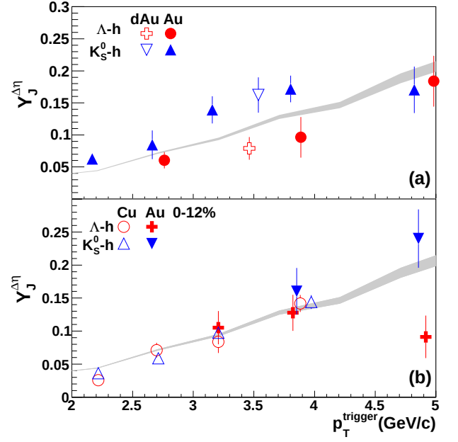
FIG. 6: (Color online.) The jet-like yield in |\Delta\eta| < 0.78 as a function of p_T^{\text{trigger}} for K_S^0 -h, and \Lambda -h correlations for 1.5 GeV/c < p_T^{\text{associated}} < p_T^{\text{trigger}} in (a) minimum bias d+Au and 40-80% Au+Au collisions at \sqrt{s_{NN}} = 200 GeV and (b) 0-60% Cu+Cu and 0-12% Au+Au collisions at \sqrt{s_{NN}} = 200 GeV. For comparison h-h correlations [9] from 40-80% Au+Au collisions are shown as a band where the width represents the uncertainty. Peripheral Au+Au points have been shifted in p_T^{\text{trigger}} for visibility. The systematic uncertainty due to the uncertainty on the associated particle's reconstruction efficiency (5%) and background level extraction (2%) are not shown.
