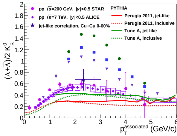
FIG. 3: (Color online.) \Lambda/K_S^0 ratio measured in the jet-like correlation in 0-60% Cu+Cu collisions at \sqrt{s_{NN}} = 200 GeV for 3 < p_T^{\text{trigger}} < 6 GeV/c and 2.0 < p_T^{\text{associated}} < 3.0 GeV/c along with this ratio obtained from inclusive p_T spectra in p - p collisions. Data are compared to calculations from PYTHIA [33] using the Perugia 2011 tunes [51] and Tune A [52].
