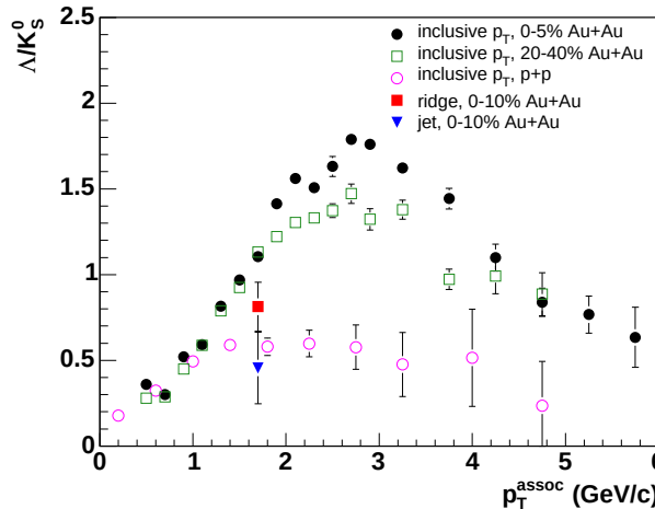
FIG. 12: \Lambda/K_S^0 ratio measured in inclusive p_T distributions, near-side jet-like and ridge-like correlation peaks in Au+Au collisions together with this ratio obtained from inclusive p_T spectra in p+p collisions.
