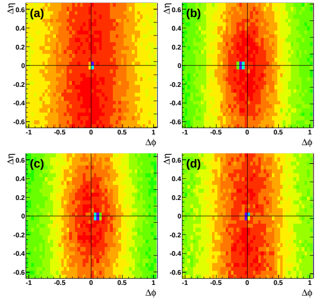
FIG. 2: The dip region in (\Delta\phi, \Delta\eta) charged-charged correlations for 3 \text{ GeV}/c < p_T^{trig} < 6 \text{ GeV}/c and 1.5 \text{ GeV}/c < p_T^{assoc} < p_T^{trig} unfolded to four helicity combinations of trigger and associated particles: (a) (h_{trig}, h_{assoc}) = (1,1) , (b) (h_{trig}, h_{assoc}) = (1,-1) , (c) (h_{trig}, h_{assoc}) = (-1,1) , and (d) (h_{trig}, h_{assoc}) = (-1,-1) .
