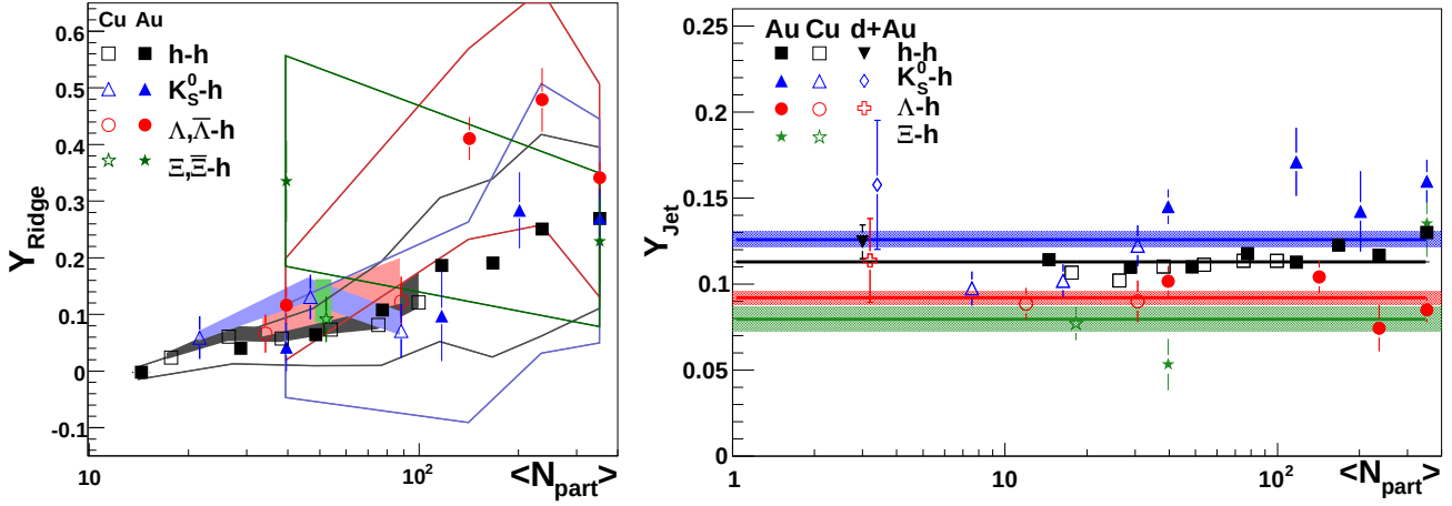
FIG. 4: Centrality dependence of the ridge yield (a) and jet-like yield (b) of associated charged particles for various trigger species in d+Au and Au+Au collisions. The error bands indicate systematic errors on the ridge yield due to the v_2 subtraction.
