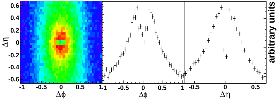
FIG. 1: (a) Two-particle di-hadron correlation function in (\Delta\phi, \Delta\eta) space for p_T^{trig}=3-6 GeV/c and p_T^{assoc} > 1.5 GeV/c in central Au+Au collisions at \sqrt{s_{NN}} = 200 GeV, not corrected for track merging. The projection of the correlation function in (b) \Delta\phi for |\Delta\eta| < 0.7 and (c) \Delta\eta for |\Delta\phi| < 0.7 . Solid line - not corrected for track merging, dashed - after the track merging correction (see text).
