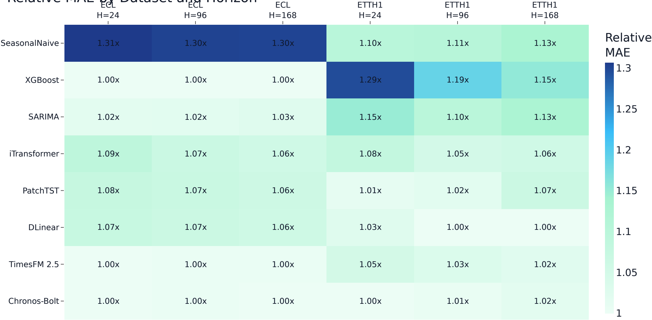
Relative MAE by Dataset and Horizon
