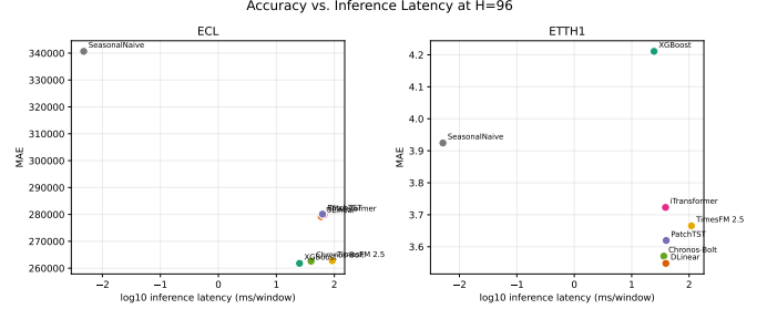
Fig. 4. Accuracy–latency view at H=96.
