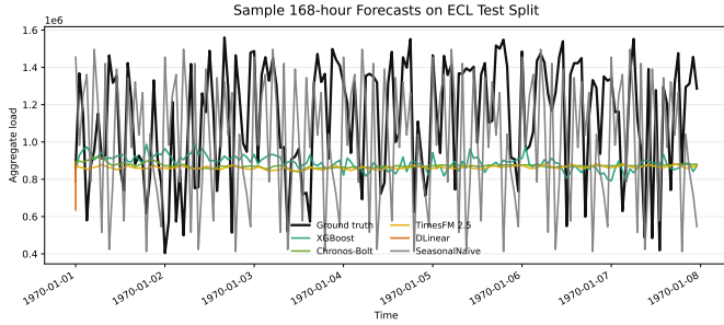
Fig. 2. Sample 168-hour ECL forecasts from representative models.
