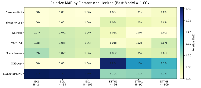
Fig. 3. MAE heatmap across executed datasets and horizons.
