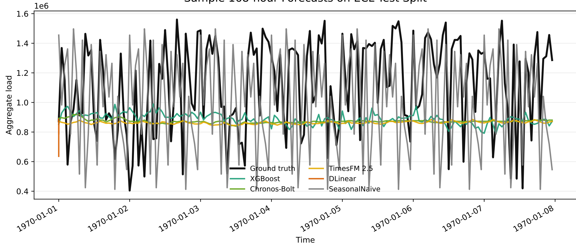
Sample 168-hour Forecasts on ECL Test Split
