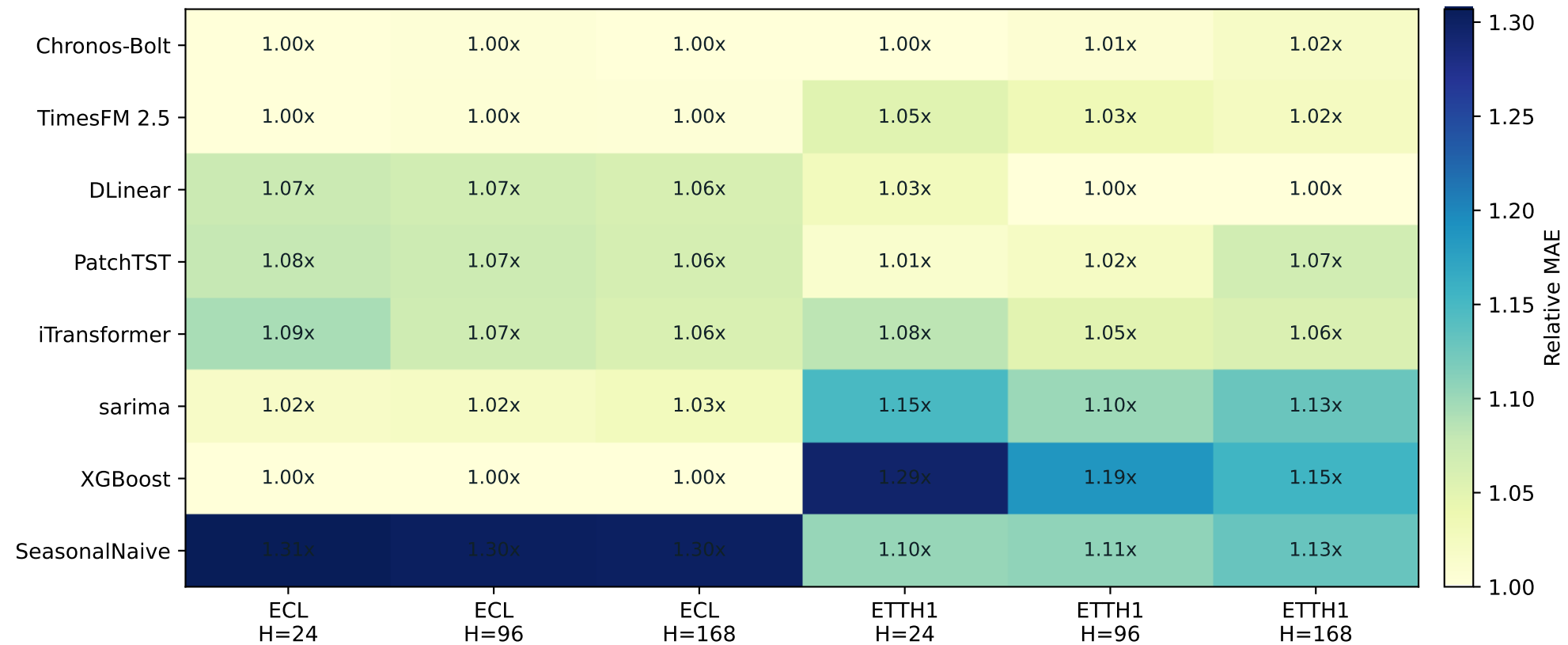
Relative MAE by Dataset and Horizon (Best Model = 1.00x)
