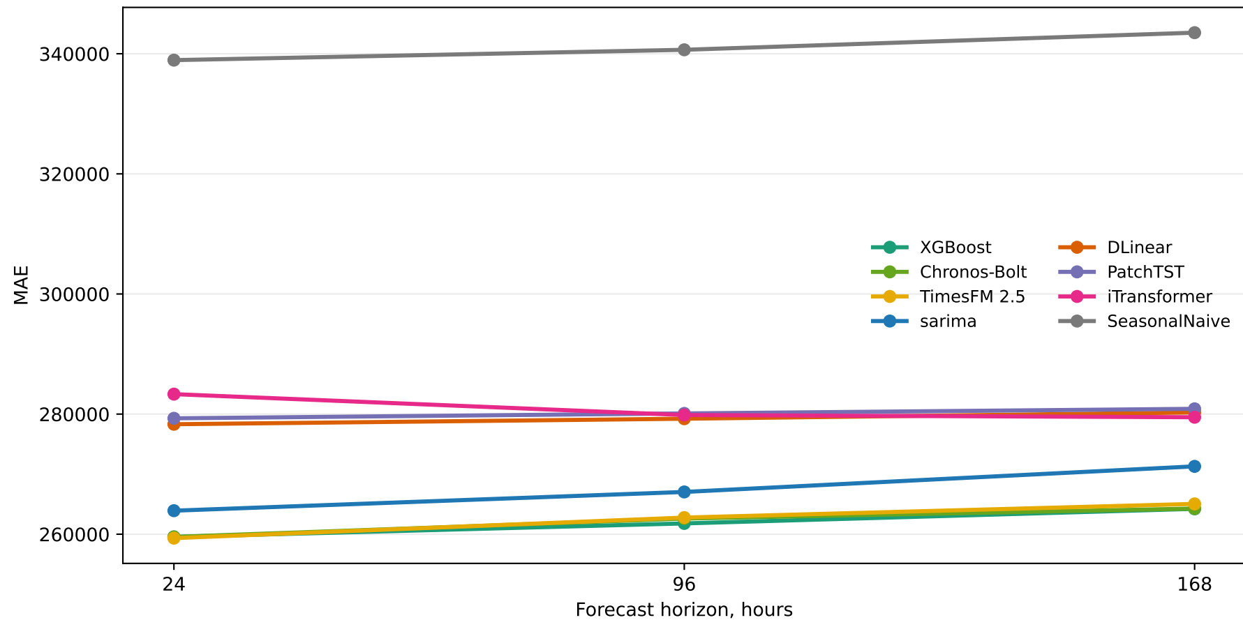
MAE Across Forecast Horizons: ECL
