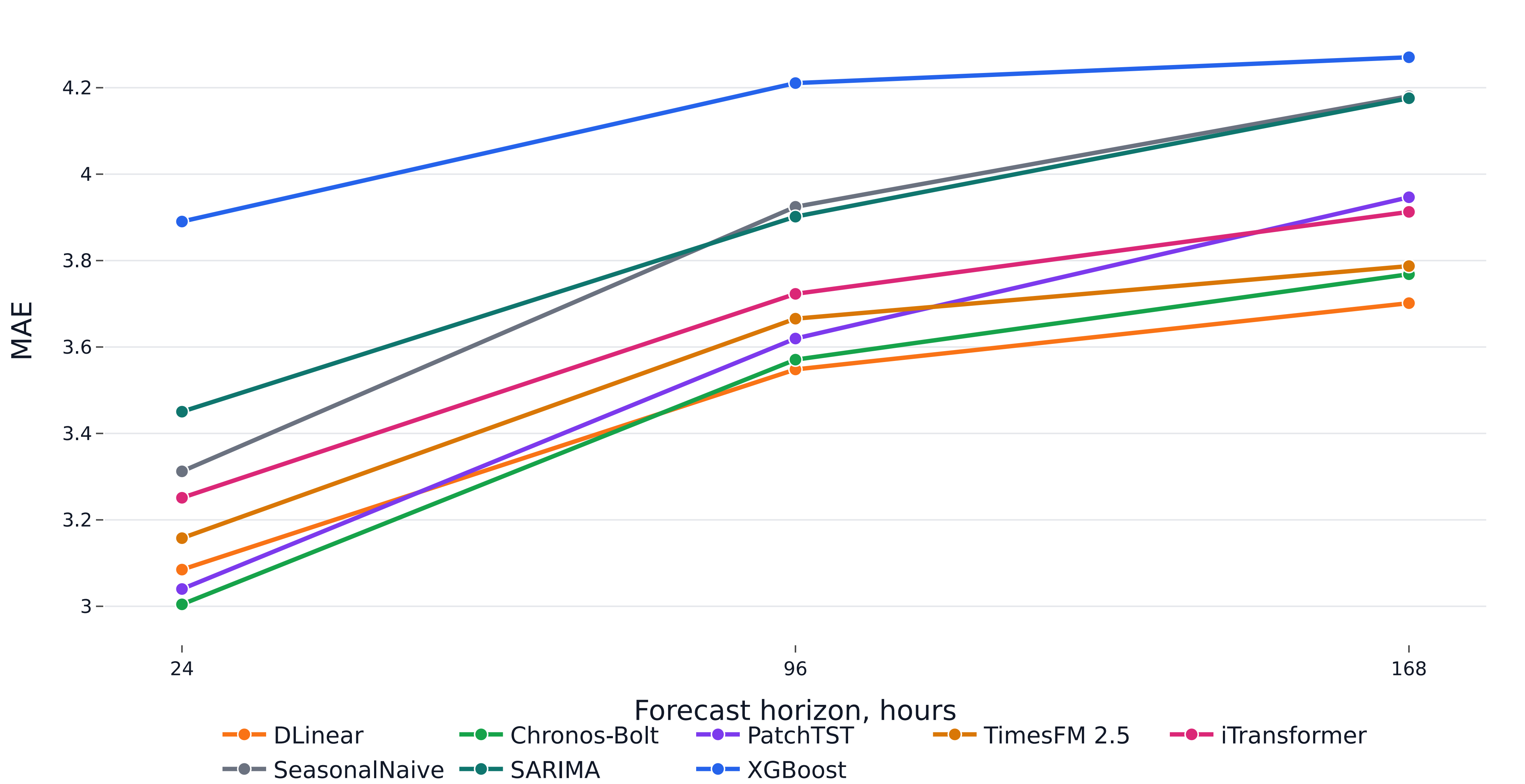
MAE Across Forecast Horizons: ETTH1
