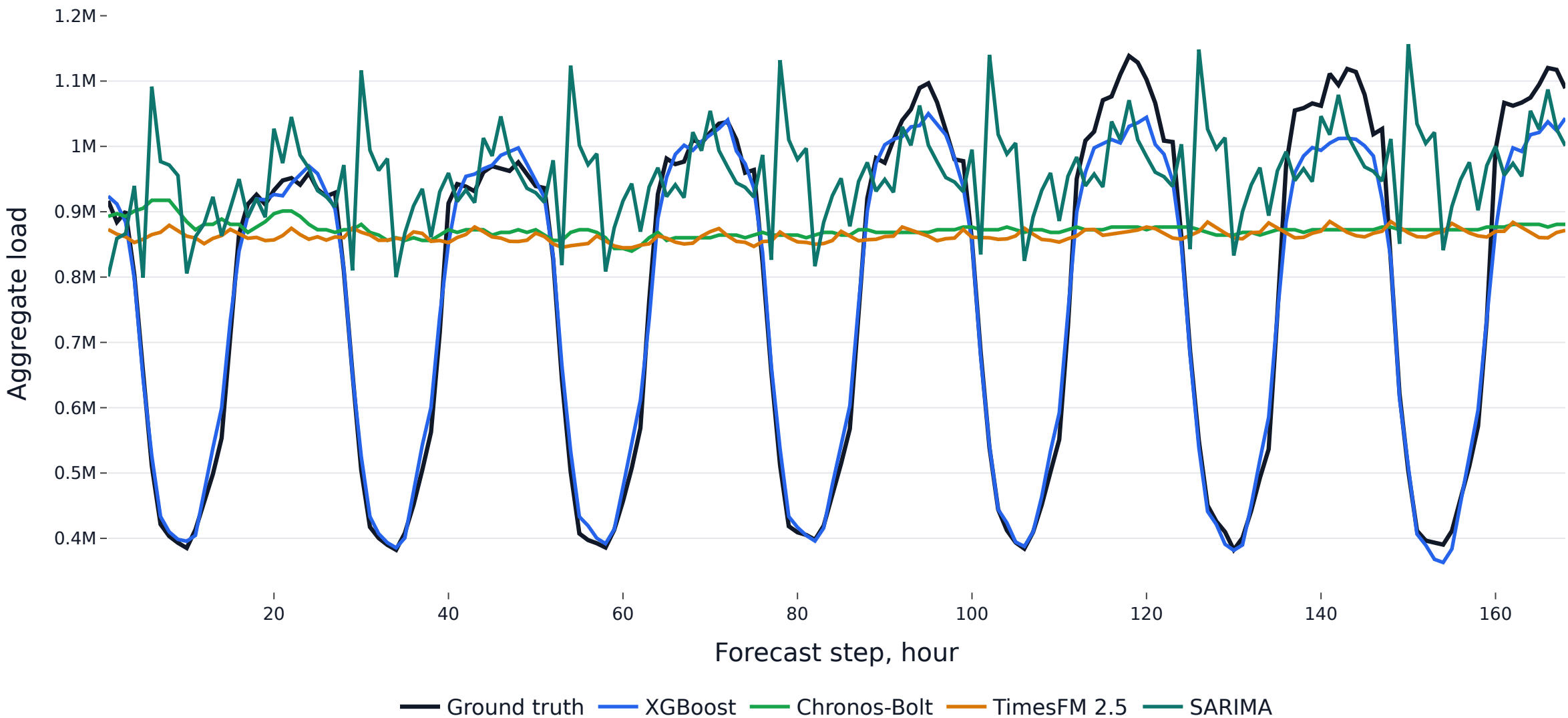
Sample 168-Hour ECL Forecast Window
