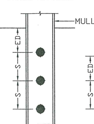
CONNECTION 11.3 SINGLE MULLION THREE ANCHORS
