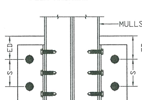
CONNECTION 11.7 DUAL MULLIONS FOUR ANCHORS
