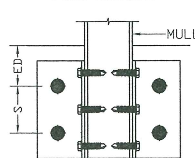
CONNECTION 11.4 SINGLE MULLION FOUR ANCHORS
