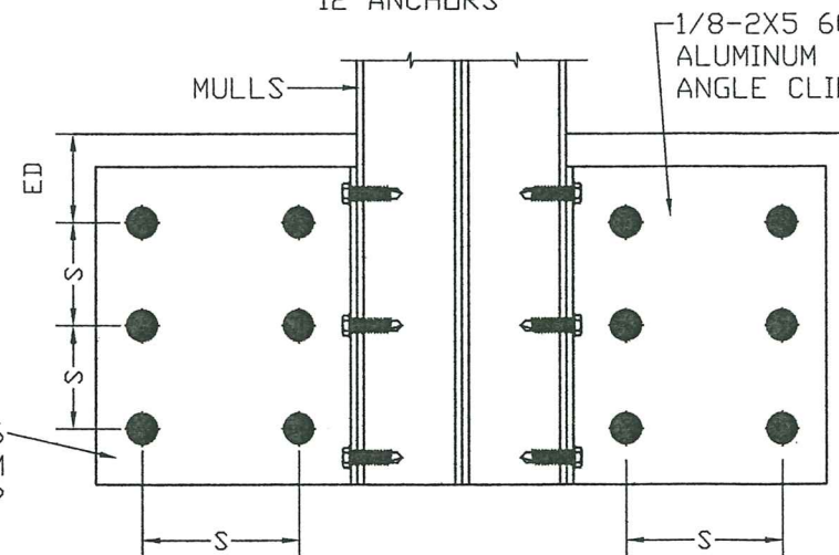
CONNECTION 11.10 DUAL MULLIONS 12 ANCHORS
