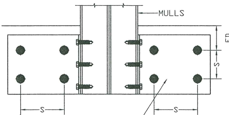
CONNECTION 11.9 DUAL MULLIONS EIGHT ANCHORS
