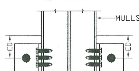
CONNECTION 11.6 DUAL MULLIONS TWO ANCHORS
