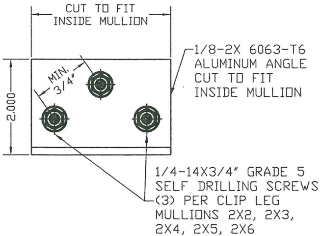
CONNECTION 9 CLIP ANCHORED TO MULLION BAR
