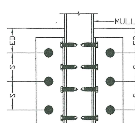
CONNECTION 11.5 SINGLE MULLION SIX ANCHORS
