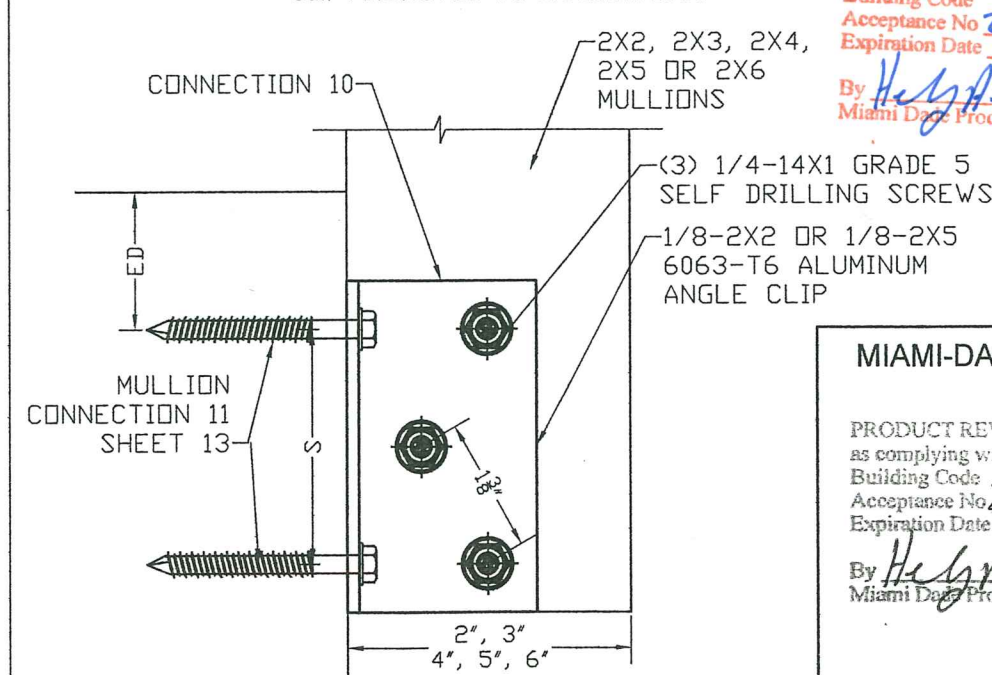
CONNECTION 10 CLIP ANCHORED TO MULLION BAR
