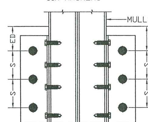
CONNECTION 11.8 DUAL MULLIONS SIX ANCHORS
