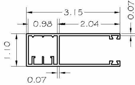
A21- GE8028 ALTERNATE SIDE RAIL COMPATIBLE WITH E555 6063-T6 ALLOY
