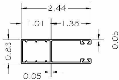
B2- GE62X21 SIDE RAIL COMPATIBLE WITH E544 6063-T6 ALLOY
