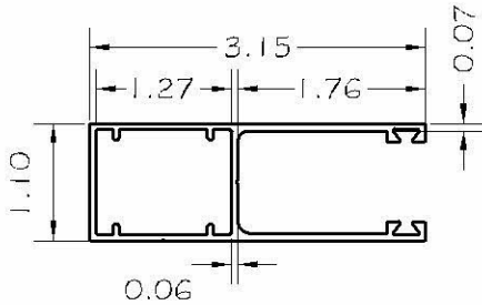
A2- GE458028 SIDE RAIL COMPATIBLE WITH E555, 6063-T6 ALLOY
