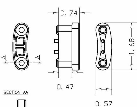
4- NYLON SLAT LOCK
