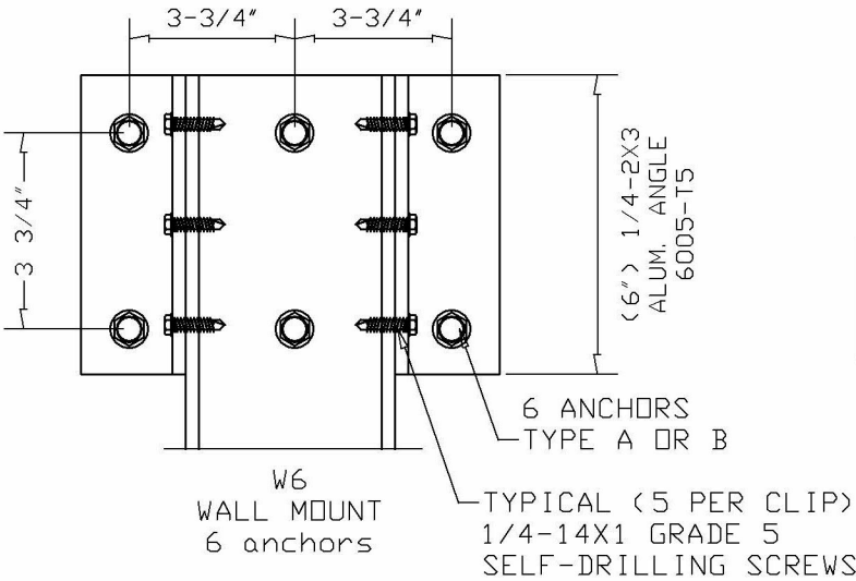
WALL MOUNT ANCHOR SELECTION
