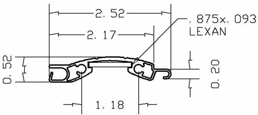
1A- ES55 LEX W/LEXAN INSERT EXTRUDED ALUMINUM 6063-T6
