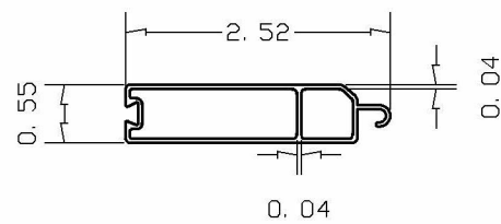
2- TE14X56U END SLAT 6063-T6 EXTRUDED ALUMINUM
