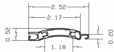
1- ES55 SUP SLAT EXTRUDED ALUMINUM 6063-T6
