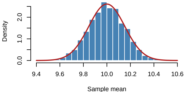
Sampling Distribution of Mean: n = 210
