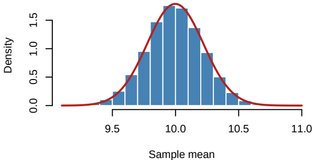
Sampling Distribution of Mean: n = 100
