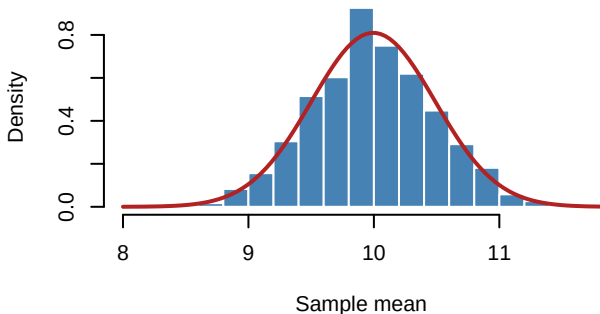
Sampling Distribution of Mean: n = 21
