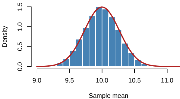
Sampling Distribution of Mean: n = 70
