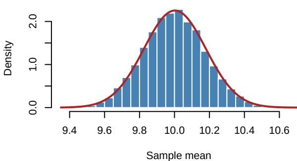
Sampling Distribution of Mean: n = 160
