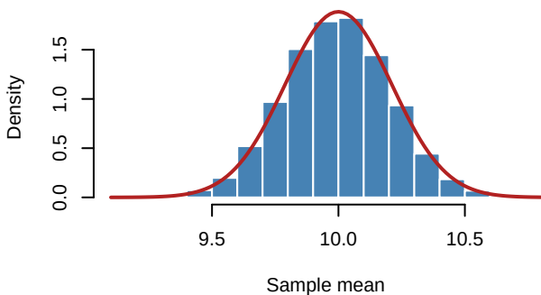
Sampling Distribution of Mean: n = 110
