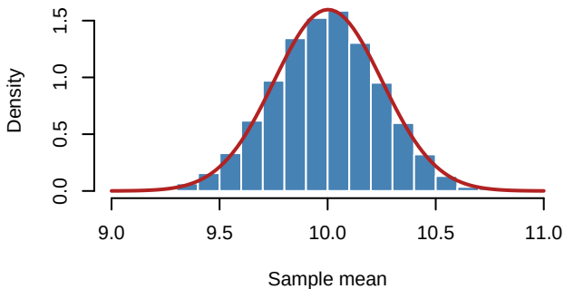
Sampling Distribution of Mean: n = 80
