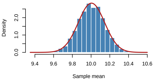
Sampling Distribution of Mean: n = 250
