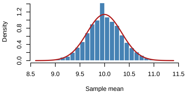
Sampling Distribution of Mean: n = 41
