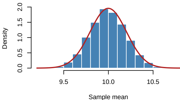
Sampling Distribution of Mean: n = 120
