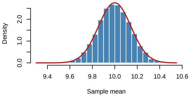
Sampling Distribution of Mean: n = 240
