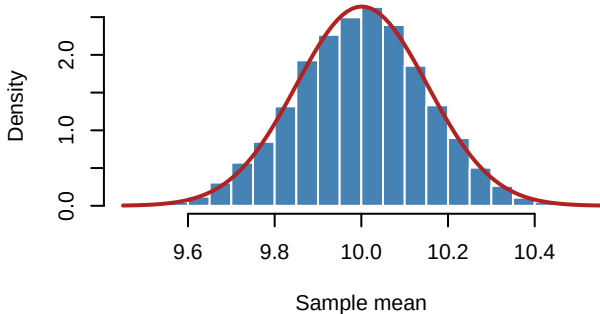
Sampling Distribution of Mean: n = 220
