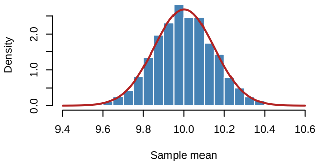
Sampling Distribution of Mean: n = 230
