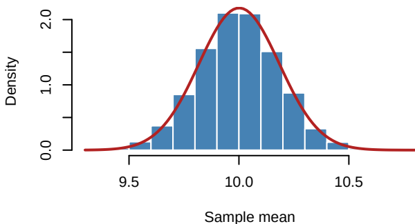
Sampling Distribution of Mean: n = 150
