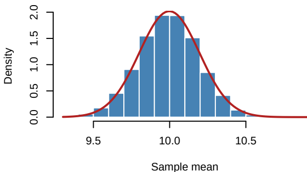
Sampling Distribution of Mean: n = 130
