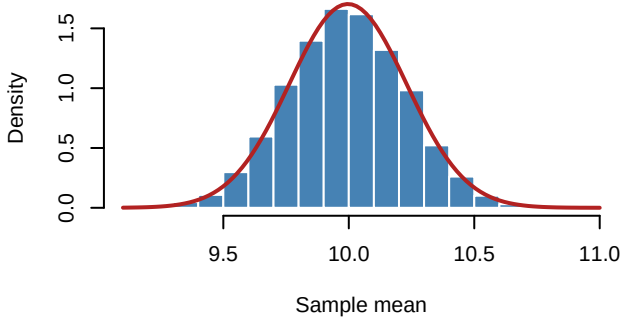
Sampling Distribution of Mean: n = 90
