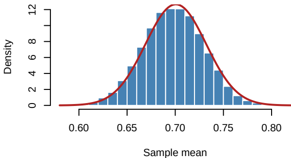
Sampling Distribution of Mean: n = 200
