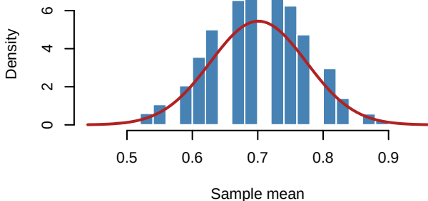
Sampling Distribution of Mean: n = 41
