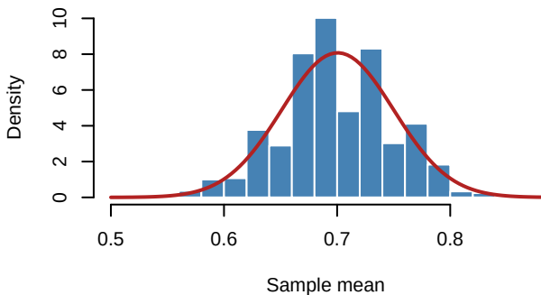
Sampling Distribution of Mean: n = 80
