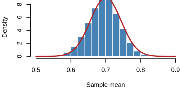
Sampling Distribution of Mean: n = 100
