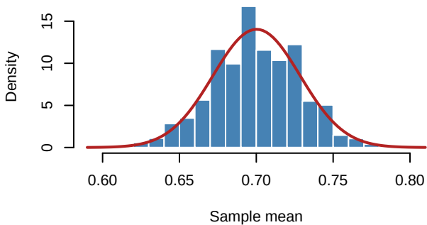
Sampling Distribution of Mean: n = 240
