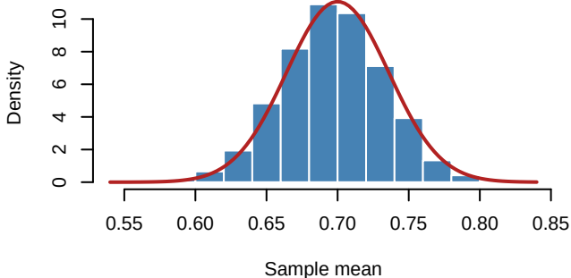
Sampling Distribution of Mean: n = 160
