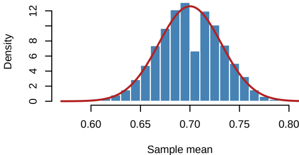
Sampling Distribution of Mean: n = 190
