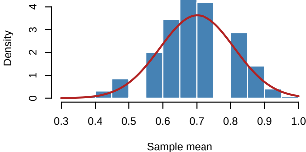
Sampling Distribution of Mean: n = 21
