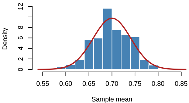
Sampling Distribution of Mean: n = 120
