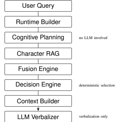
Fig. 3. Query pipeline: user queries are processed through runtime construction, language-model-free cognitive planning, retrieval-augmented generation, multi-source fusion, deterministic decision scoring, context assembly, and terminal language model verbalization. The language model is invoked exactly once, at the final stage.
