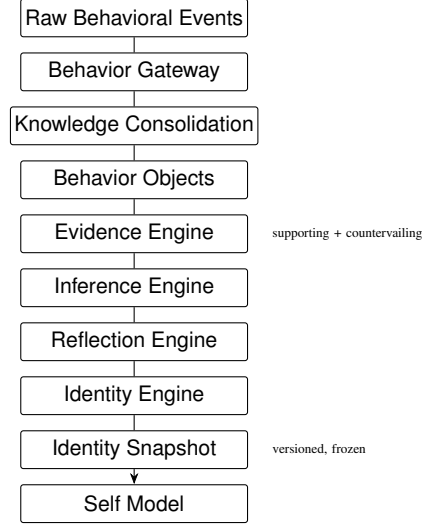
Fig. 2. Identity construction pipeline: raw behavioral events are normalized, consolidated into behavior objects, processed through evidence and inference engines with counter-evidence tracking, assembled into a structured identity, frozen into immutable snapshots at evolutionary thresholds, and exposed through a self-model with uncertainty quantification.
