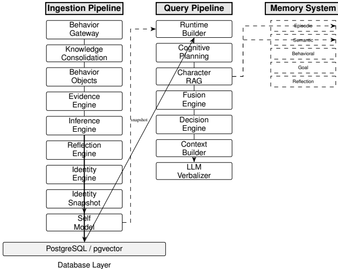
Fig. 1. AIMirror architecture: two-pipeline layout with ingestion (behavioral observation to identity construction) and query (user request to verbalized response) pipelines, connected via frozen identity snapshots. Fusion Engine merges multi-source retrieved items before deterministic selection. The memory system provides five specialized storage types accessible to the retrieval components.
