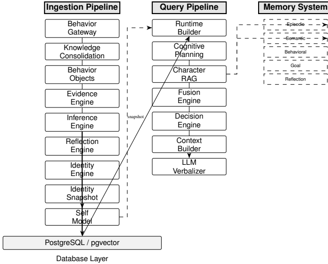
Fig. 1. AIMirror architecture: two-pipeline layout with ingestion (behavioral observation to identity construction) and query (user request to verbalized response) pipelines, connected via frozen identity snapshots. Fusion Engine merges multi-source retrieved items before deterministic selection. The memory system provides five specialized storage types accessible to the retrieval components.
