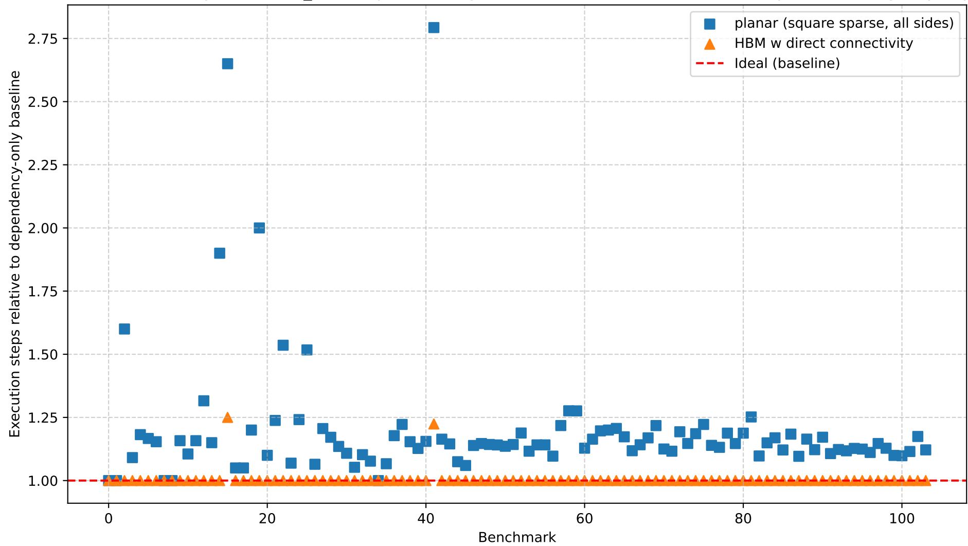
HBM with direct connectivity (hbm arch_A) over planar (magic) normalized to ideal execution steps considering only dependencies
