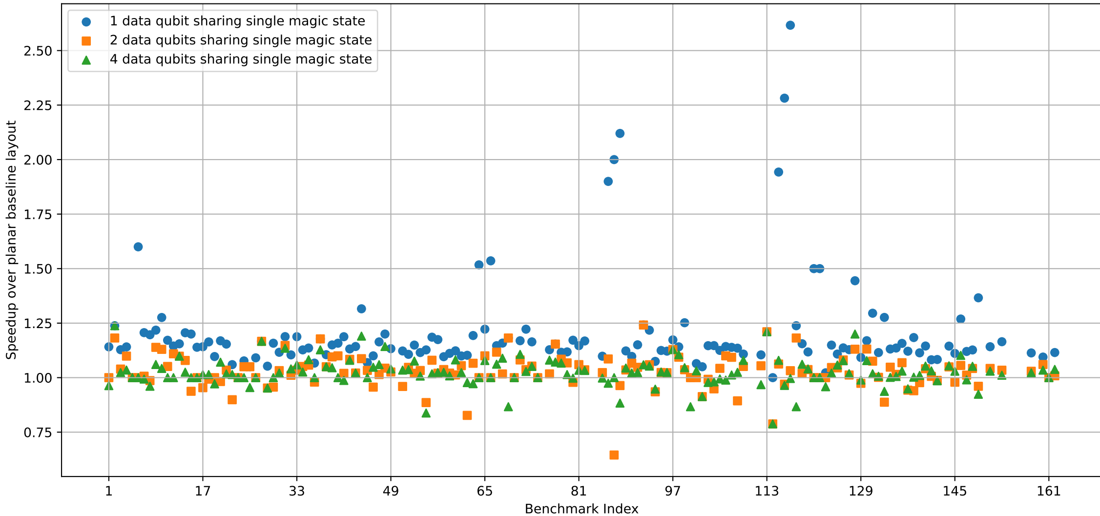
Effect of different numbers of data qubits sharing a single magic state (routing on lower level)
