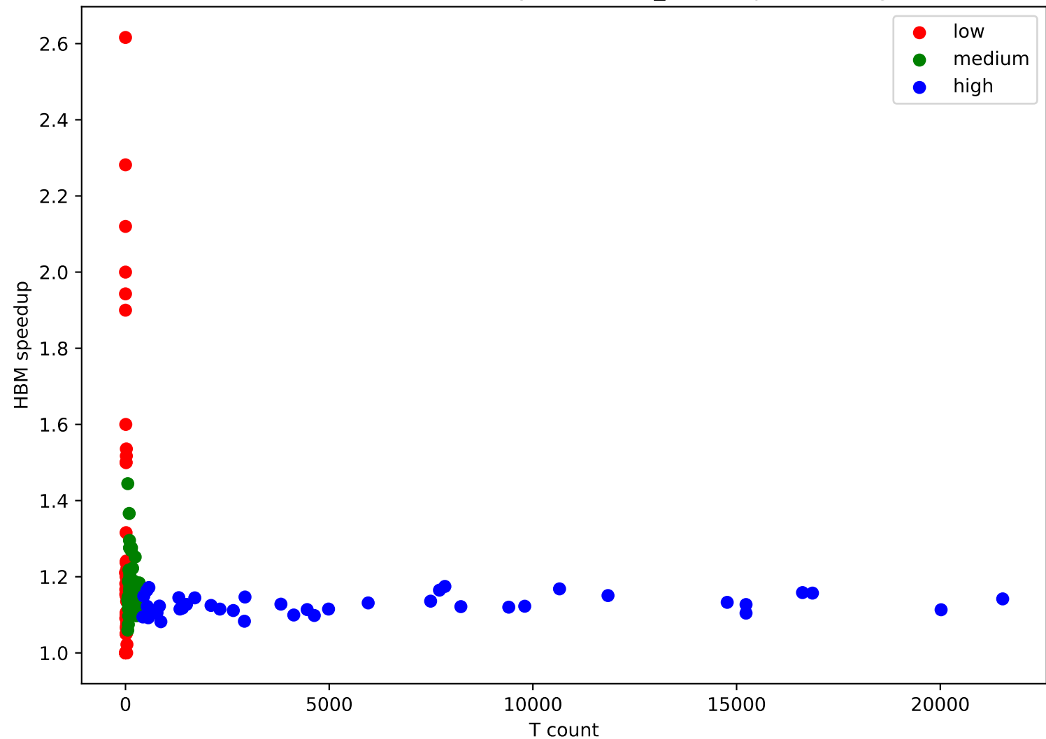
HBM with direct connectivity (hbm arch_A) over planar (magic)
