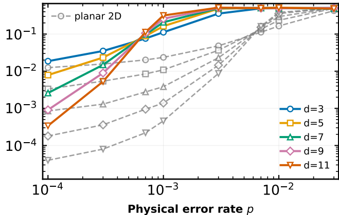
HBM - vertical coupling error rate p' = 10p
