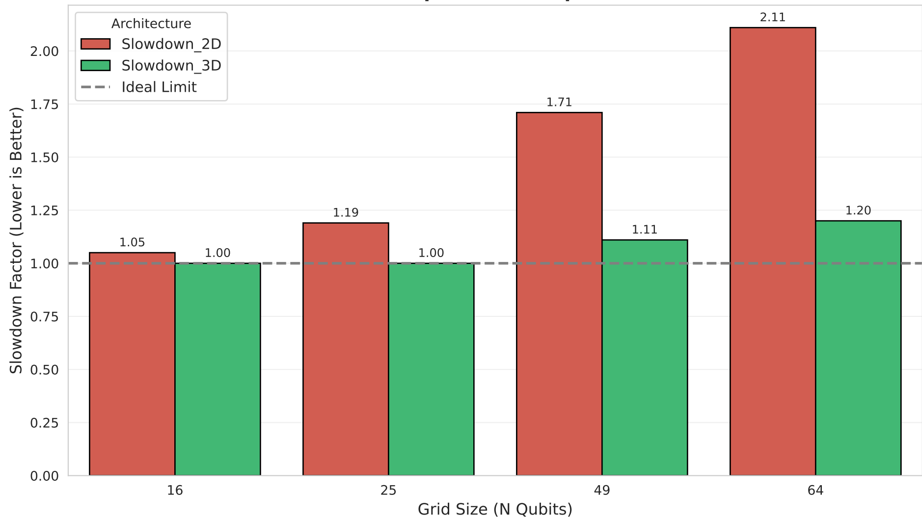
Slowdown Factor for Deep Circuits (Depth L=100, Traffic P=0.5)
