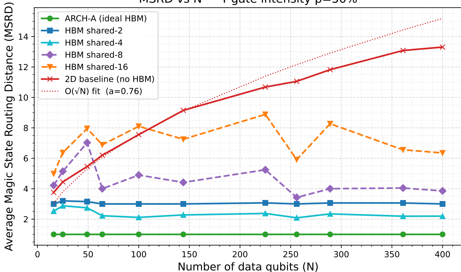
MSRD vs N — T-gate intensity p=50%
