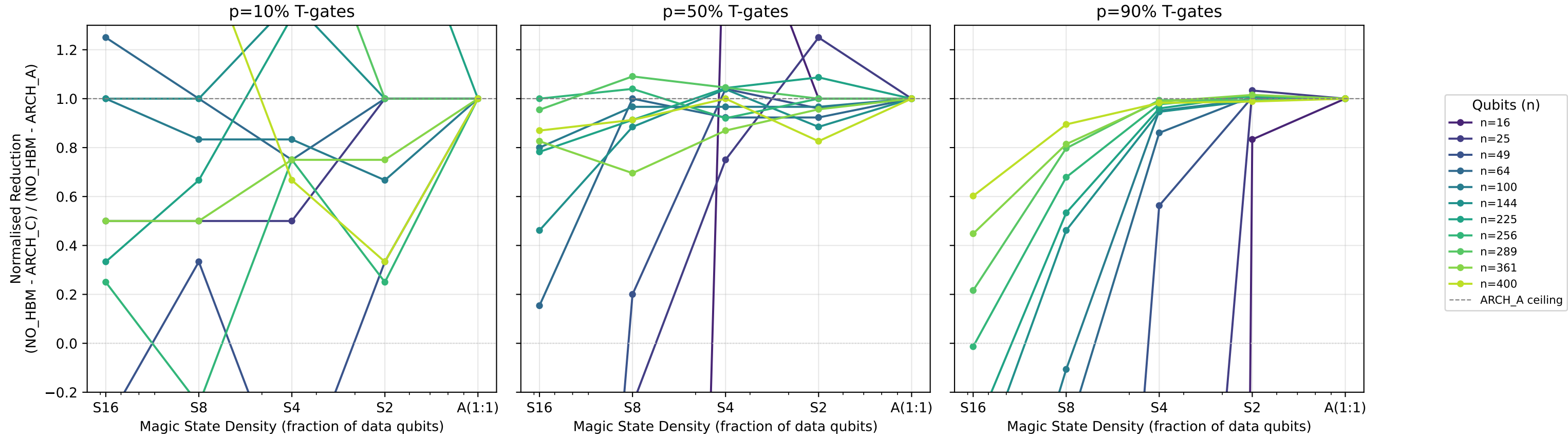
HBM Trade-off: Magic State Density vs Normalised Timestep Reduction
