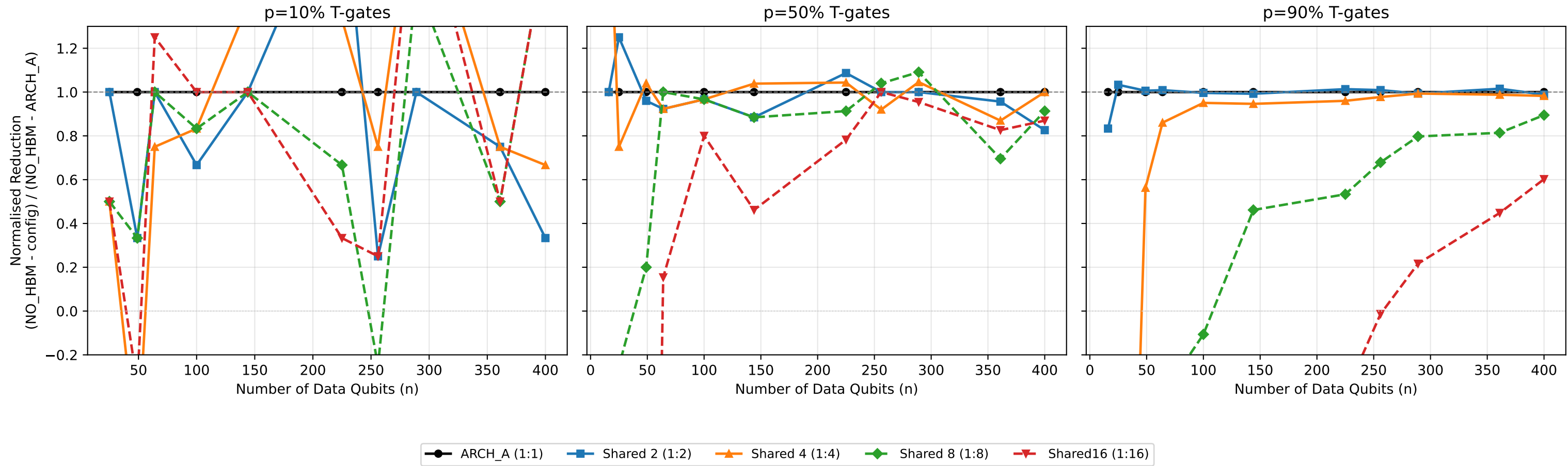
HBM Benefit Scaling with Qubit Count
