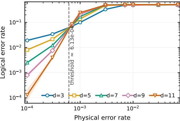
HBM - vertical coupling error rate p' = 10p
