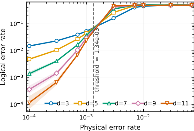
HBM - vertical coupling error rate p' = 5p
