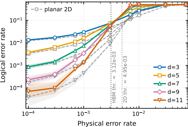
HBM - vertical coupling error rate p' = p
