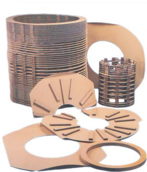
PRESSURE RINGS SPACERS AND COMPENSATORS
