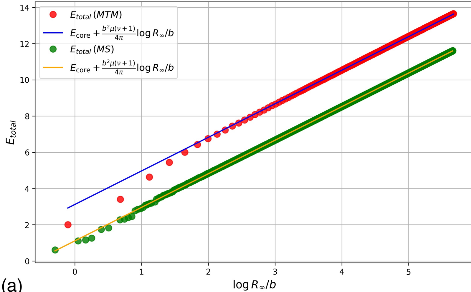
Dislocation Core Energy (MS vs MTM)
