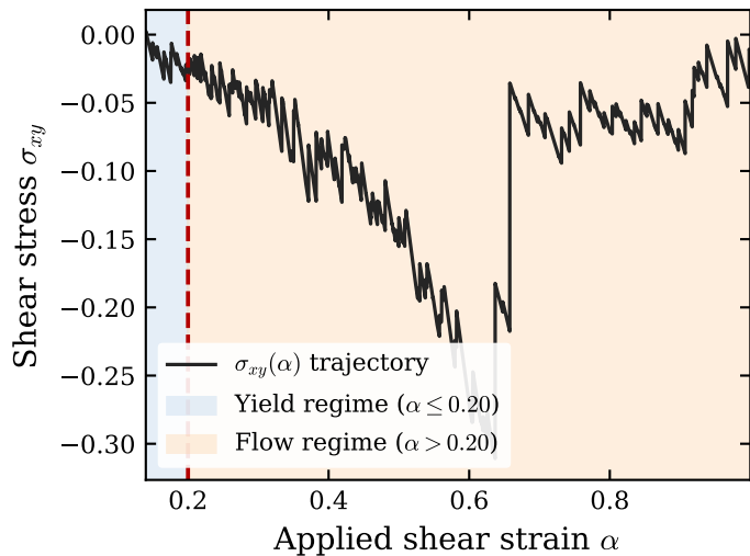
(a) Shear Stress Trajectory & Yield
