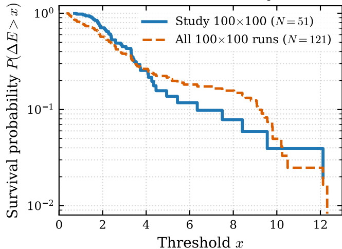
(c) Exceedance Probability (CCDF)
