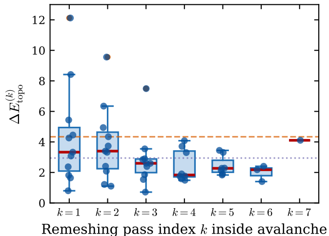
(b) Jump Size Across Surgery Passes
