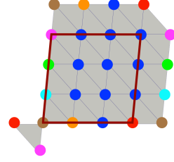
FIG. 2. The periodicity unit of the computational mesh \mathcal{T}_{\text{ch}} obtained by periodic Delaunay triangulation. The central computational domain \Omega_0 is limited by the brown box. Only triangles with at least one vertex in \Omega_0 are selected for the mesh (shown by the thin lines), ensuring proper connectivity across periodic boundaries while avoiding redundant counting of triangles.
