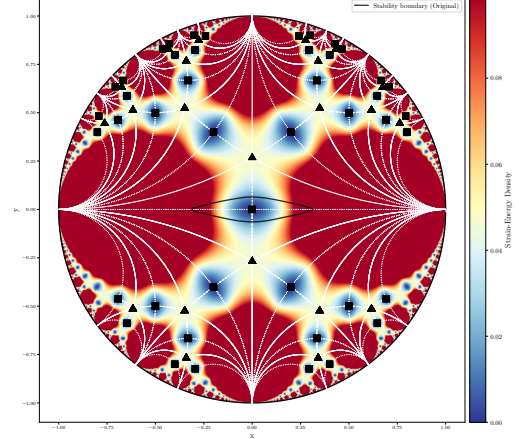
FIG. 1. Strain-energy density landscape in the the space of shear strains visualized on a Poincaré disk using stereographic projection. Thin white lines show the original tessellation into equivalent periodicity domains. Colors represent level of energy. The stability boundaries obtained from the equation (10) are shown by a thick black line around the reference energy well.)
