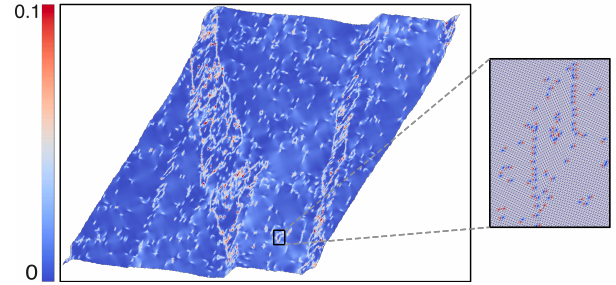
FIG. 5. The micro-configuration configuration corresponding to the state C marked in Fig. 4. Colors indicate the magnitude of strain-energy density. The inset shows a single grain and details the dislocation structure of the grain boundaries.
