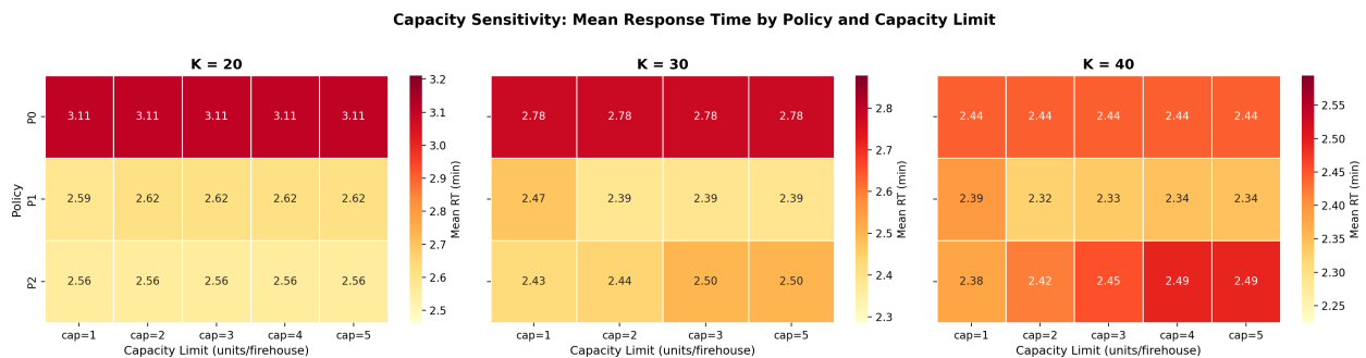
Figure 9: Capacity sensitivity heatmap showing mean response time (with 95% CI) by policy and per-firehouse capacity limit at K=20 , K=30 , and K=40 . At K=20 , capacity is non-binding for all policies — performance is essentially identical across \text{cap}=1 through \text{cap}=5 . At K=30 and K=40 , higher capacity allows concentration into fewer stations, with marginal RT effects ( < 0.15 min). This supports the decision to use \text{capacity}=2 as the operational default.
