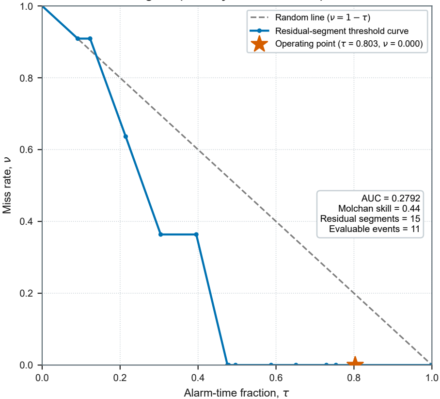
Molchan error diagram (365-day alarm windows)
