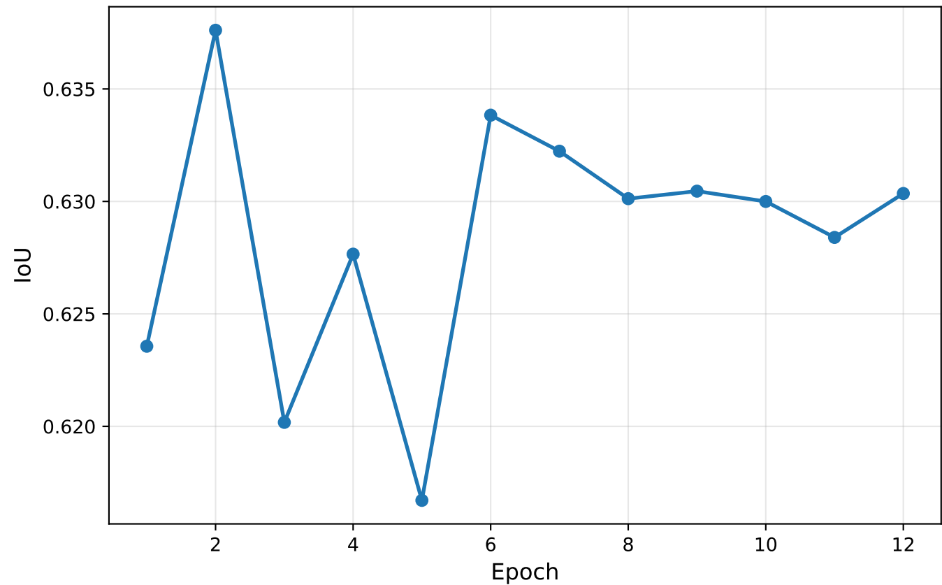
Validation IoU Performance
