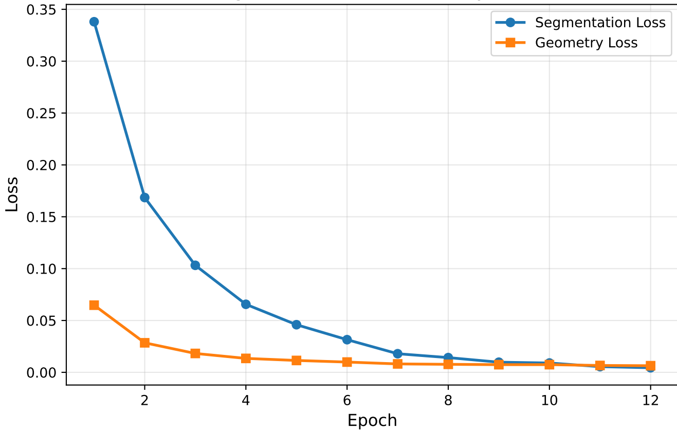
Segmentation and Geometry Loss
